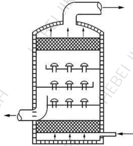
Distillation column.
